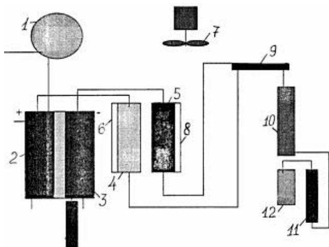
Fig. 4. – Schematic representation of an electrolysis device for producing the DDW: 1 – the atmospheric moisture condensate container; 2 – the anode; 3 – the cathode; 4 – the oxygen drier; 5 – the reactor of isotope D_2/H_2^{16}O exchange; 7 – fan; 6, 8 – ion exchange membranes; 9 – the catalytic burner; 10 – the capacitor; 11 – the water conditioning unit with dolomite; 12 – a collector of the DDW
