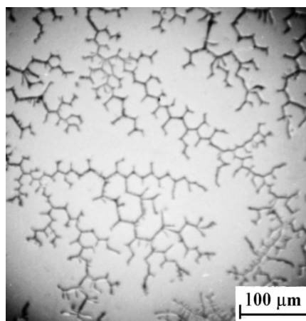
Fig. 6. Photo of the film obtained from solution containing HSA + 20 mM KCl; T = 40^{\circ}\text{C} , \text{RH}=0\% , peripheral part of the cuvette.
